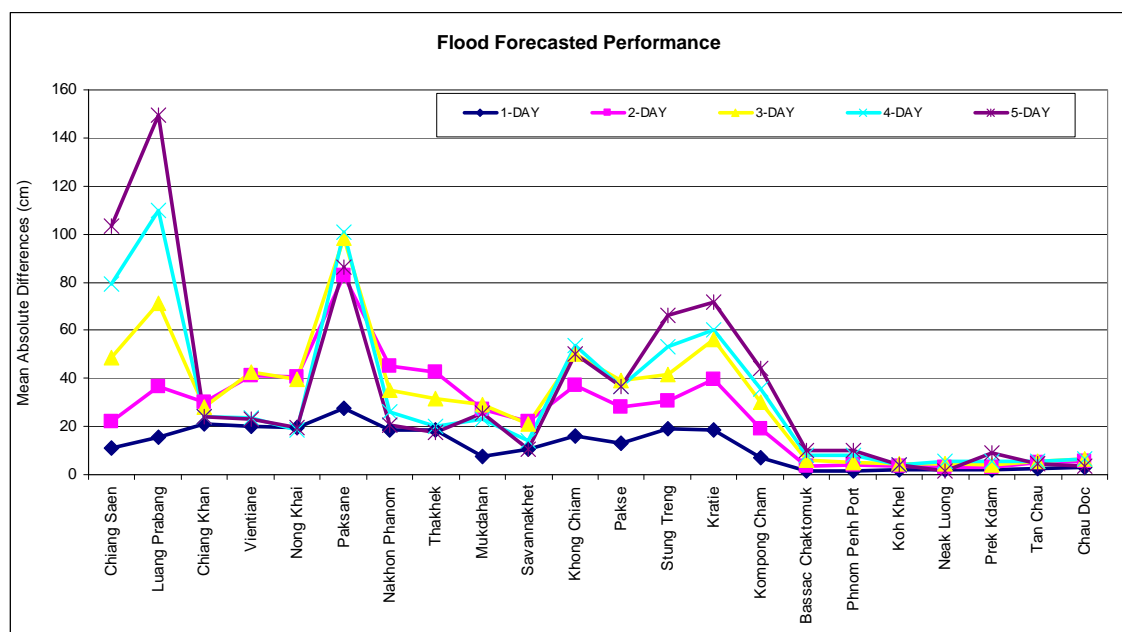
Figure B1: Average flood forecast accuracy along the Mekong mainstream (from 02 nd – 09 th October 2017)
